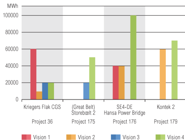
Figure 109 RES increase results for projects in the cross section between the Nordic and Continental European synchronous areas.
