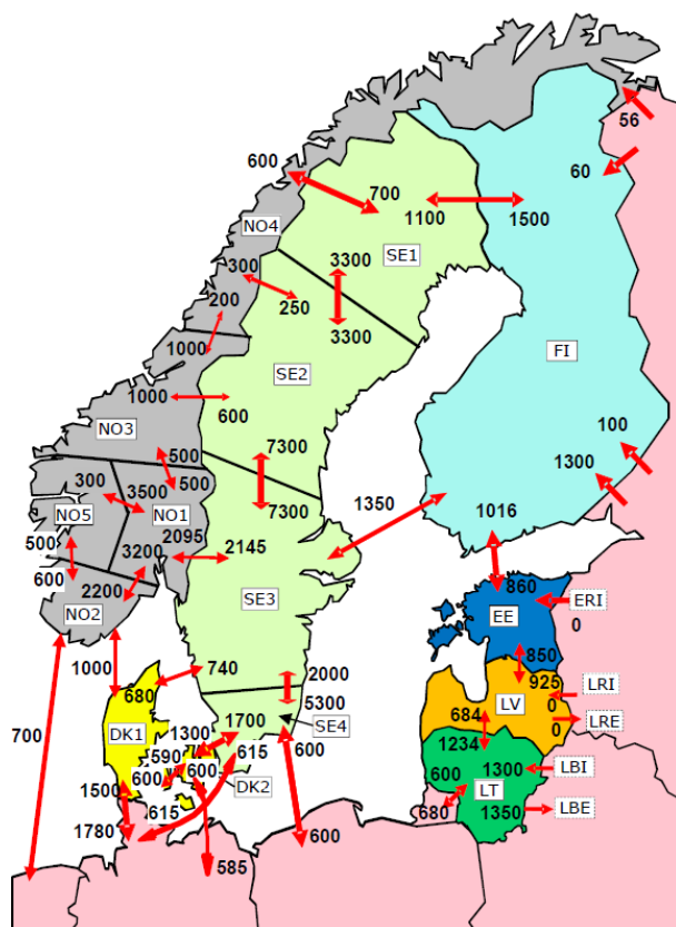
Figure 40 Illustration of Net Transfer Capacities in BS region (April 2014). Source: Nordpool Spot
