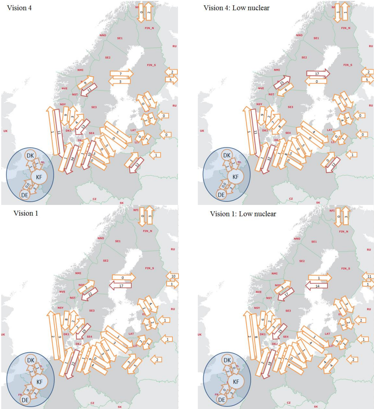
Figure 105 Energy flows in TWh; comparison of reference case with sensitivity case, Visions 1 and 4.
