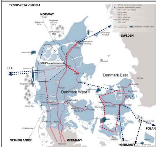
Figure 99 Study Case 1 illustration. Representation of the network reinforcements and step results in flow durations comparison vs. the given limits.
