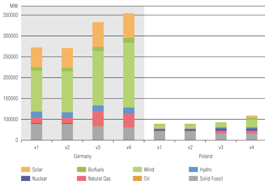
Figure 87 Generation portfolio mixture in Germany, Poland for each Visions 1, 2, 3 and 4, installed generation capacity in MW
