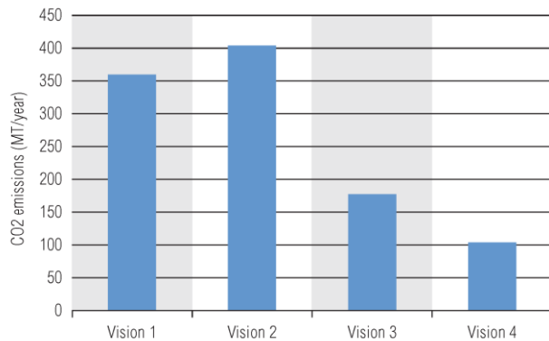
Figure 81 CO2 emissions for Baltic Sea region in all Visions
