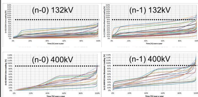
Figure 99 Study Case 1 illustration. Representation of the network reinforcements and step results in flow durations comparison vs. the given limits.
