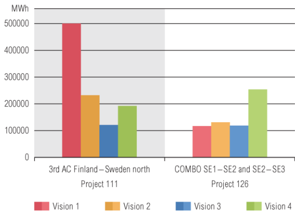
Figure 116 Increase in losses for internal projects in the Nordic synchronous area.
