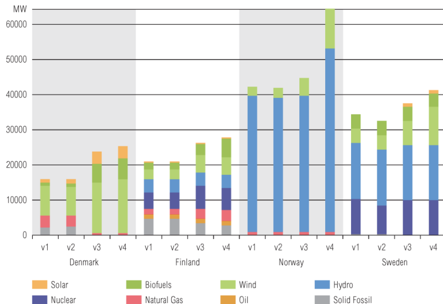
Figure 86 Generation portfolio mixture in Nordic countries for each Visions 1, 2, 3 and 4, installed generation capacity in MW.
