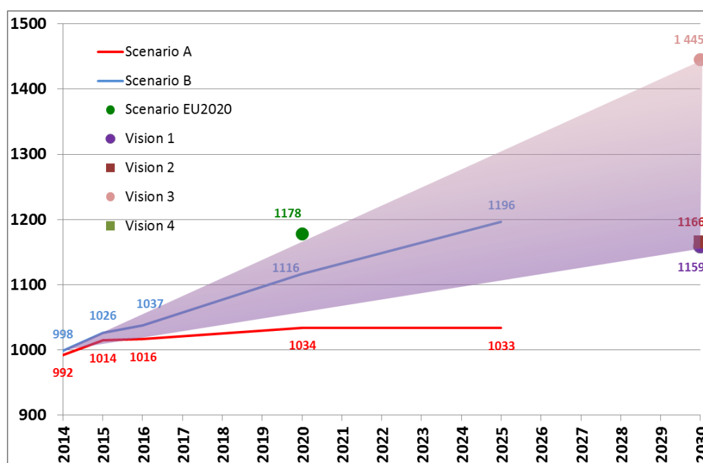
Figure 1.2: ENTSO-E total NGC development (all Scenarios; January 7 p.m.; GW)
