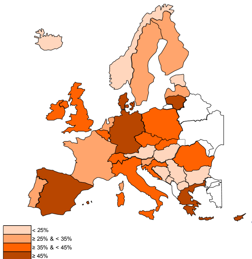
F. 3.3.10 – UC as a part of NGC per country in 2030, Vision 1, January
