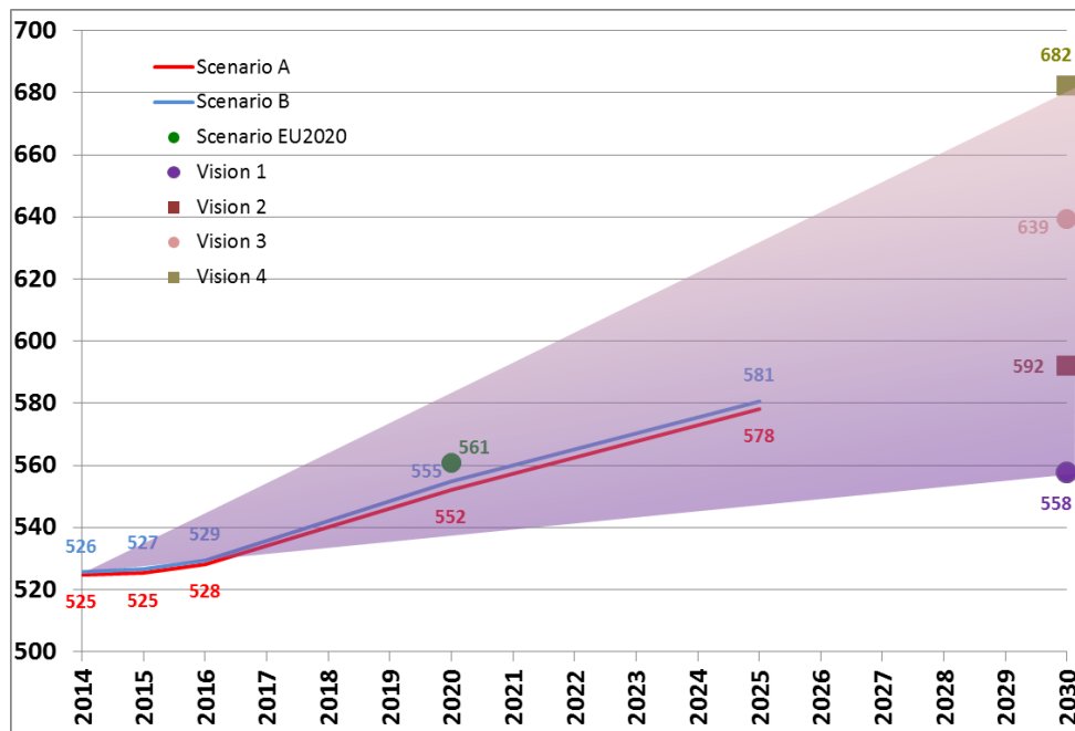
F. 3.1.1. - ENTSO-E load forecast for all scenarios in January [GW]
