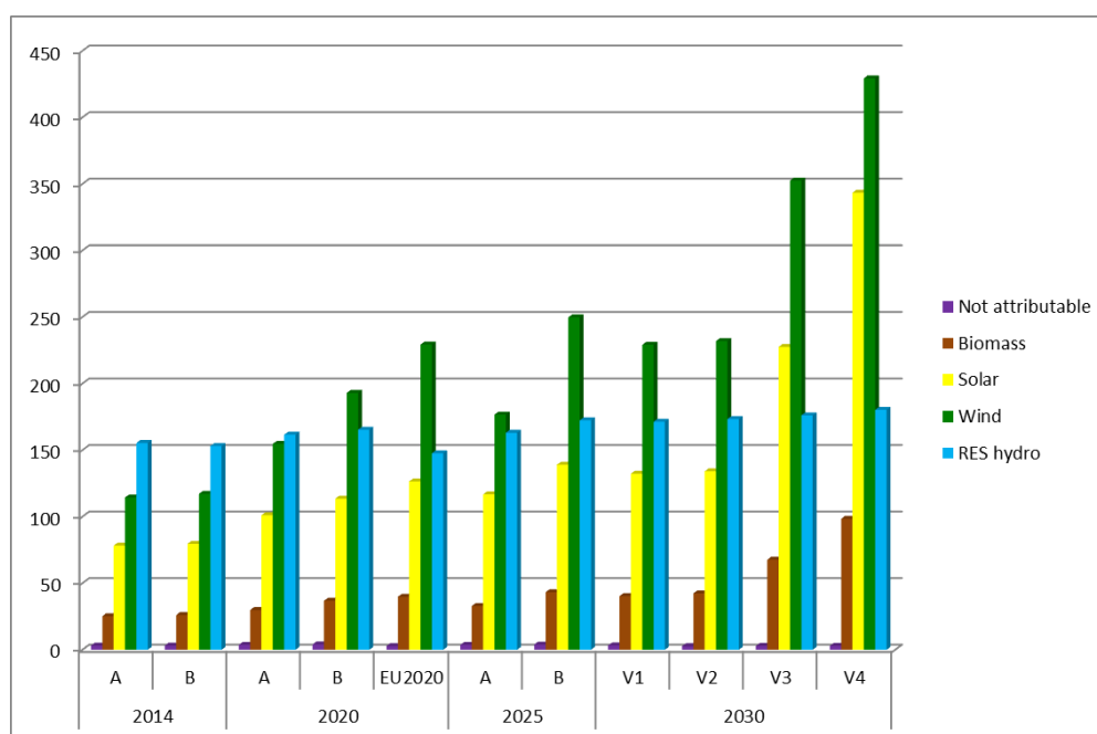
F. 3.2.4.3 – ENTSO-E RES generation capacity breakdown; all scenarios; January 7 p.m.
