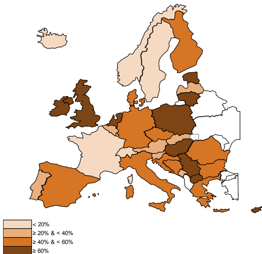
F. 3.2.2.5 - Fossil fuels installed capacity as a part of NGC per country in 2014; Scenario B; January 7 p.m.
