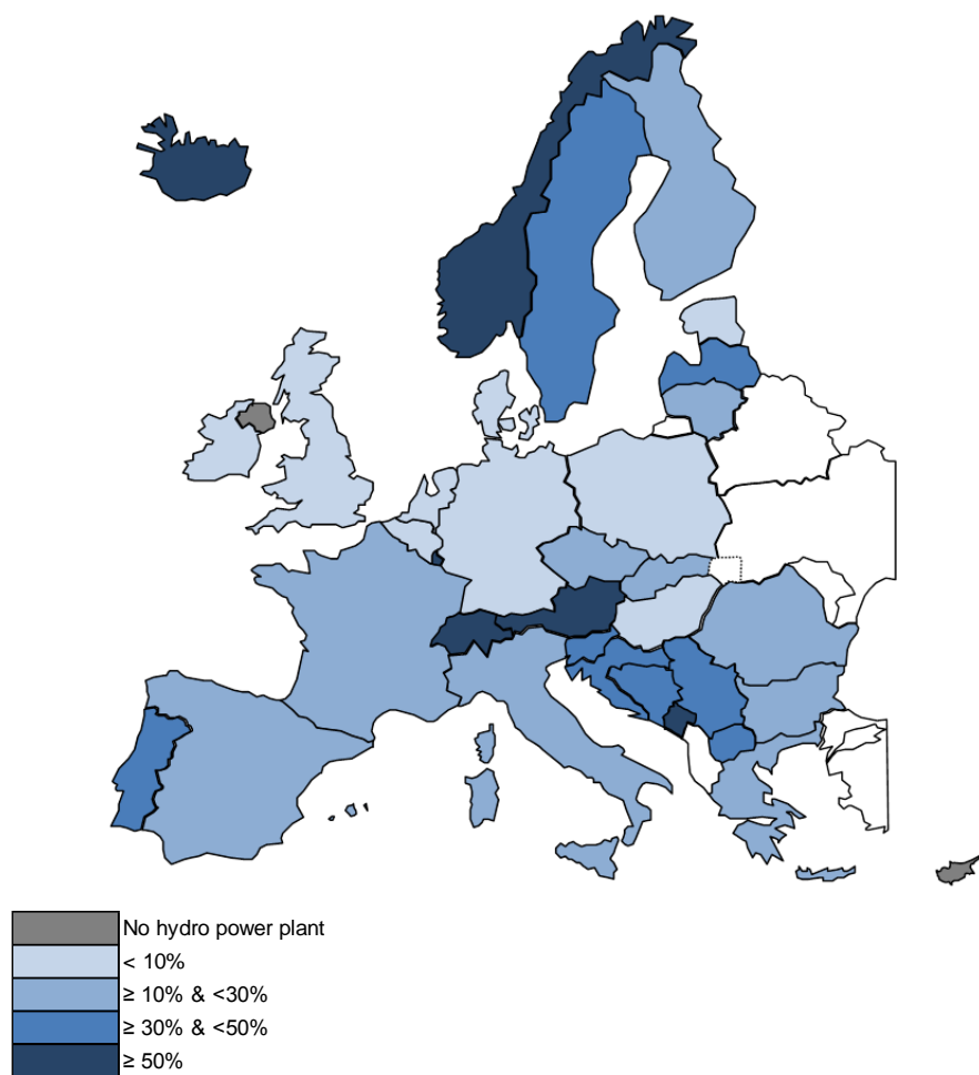
F. 3.2.5.7 – Total HPP installed capacity as part of NGC per country in 2025; Scenario B; January 7 p.m.
