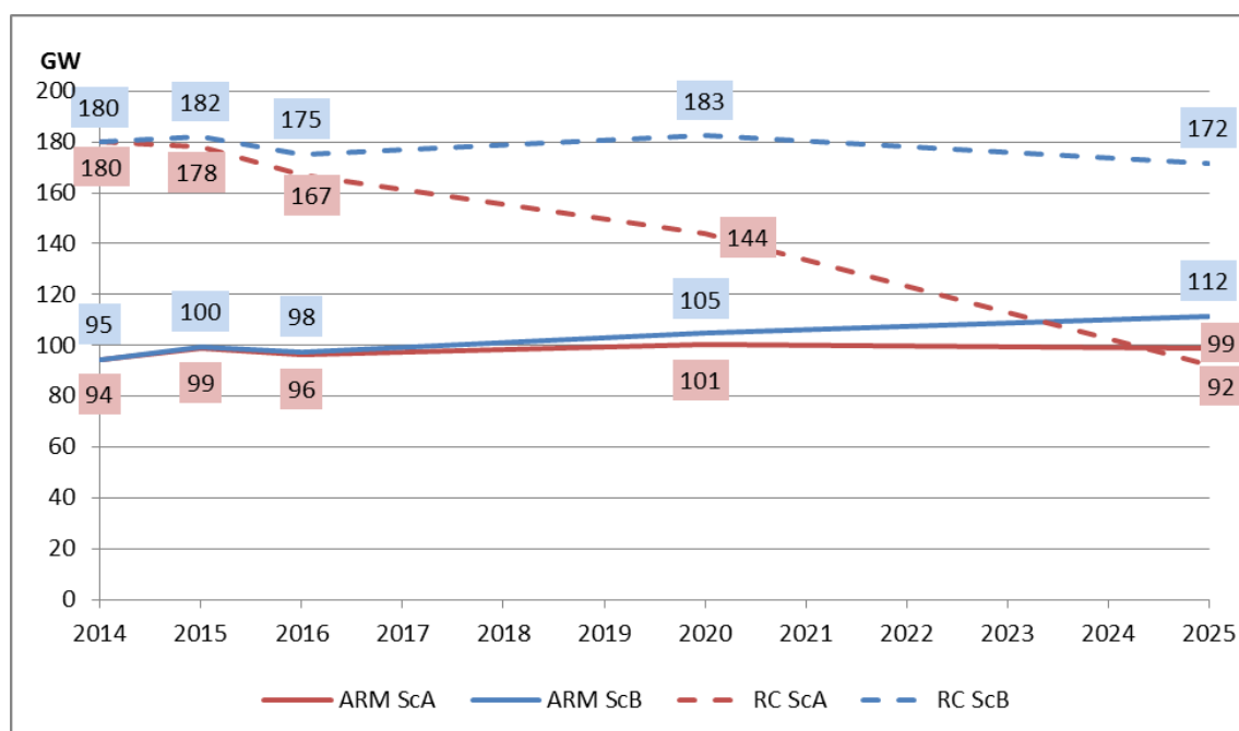
F 4.1.6 – ENTSO-E RC and ARM comparison, Scenarios A&B, July 11 a.m.
