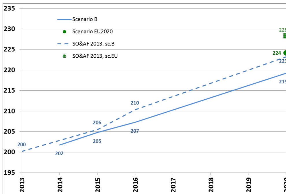
F 3.2.5.2 – Comparison of total HPP generation capacity between SO&AF 2013 and SO&AF 2014; Scenarios B and EU2020; January 7 p.m. [GW]
