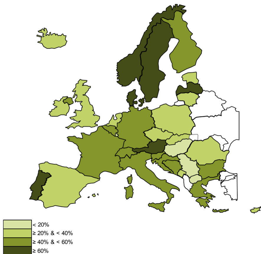
F. 3.2.4.8 – RES installed capacity as part of NGC per country in 2020; Scenario EU2020; January 7 p.m.
