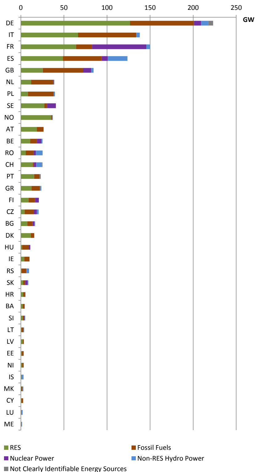
F. 3.2.1.10 – Total NGC breakdown per country in 2020; Scenario EU 2020; January 7 p.m.
