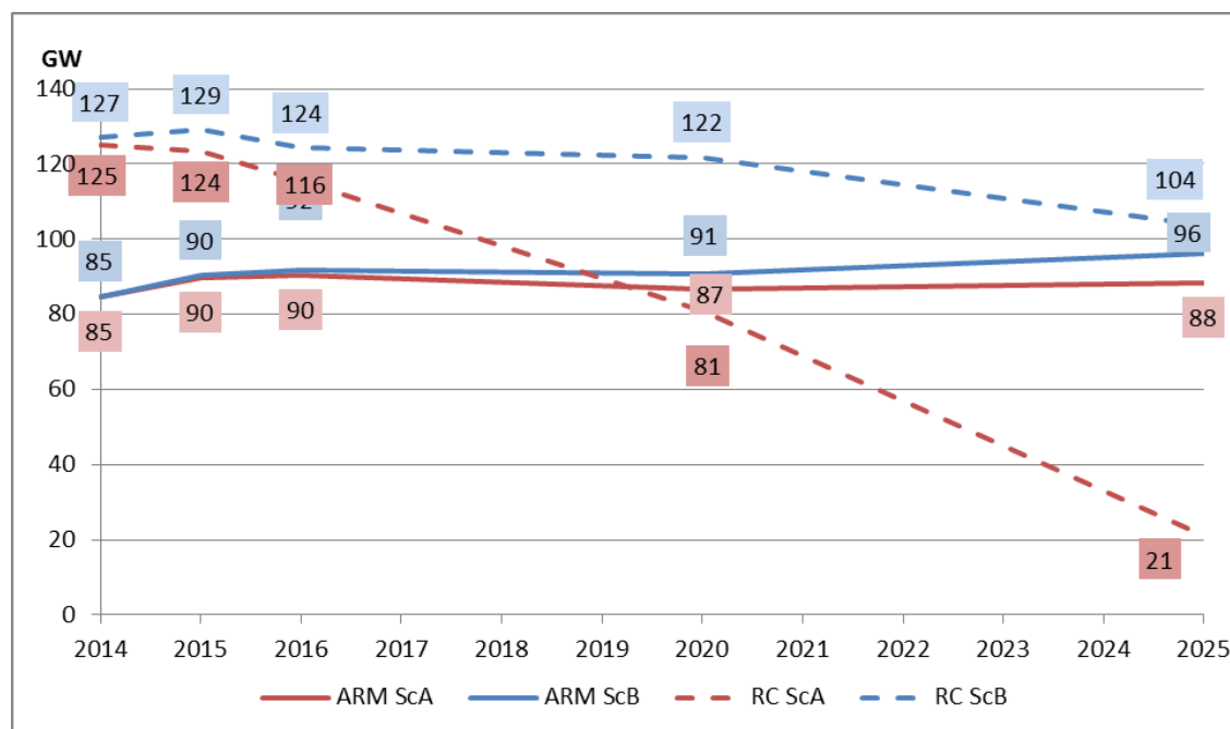
F 4.1.5 – ENTSO-E RC and ARM comparison, Scenarios A&B, January 7 p.m.
