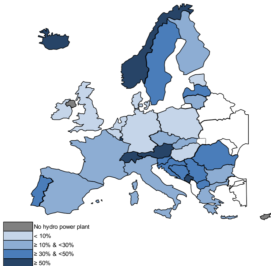
F. 3.2.5.8 – Total HPP installed capacity as part of NGC per country in 2020; Scenario EU2020; January 7 p.m.
