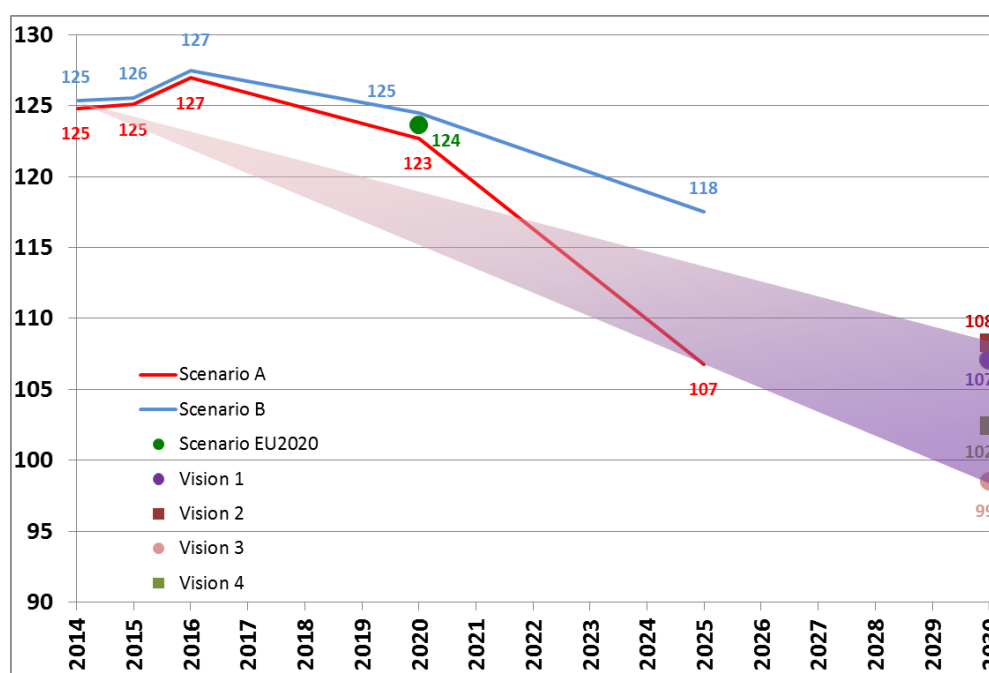
F. 3.2.3.1 – ENTSO-E Nuclear generation capacity forecast; all scenarios; January 7 p.m. [GW]
