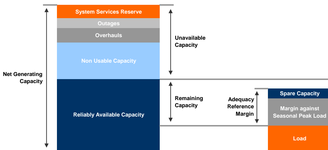
Figure 7.3: Schematic depiction of adequacy methodology
