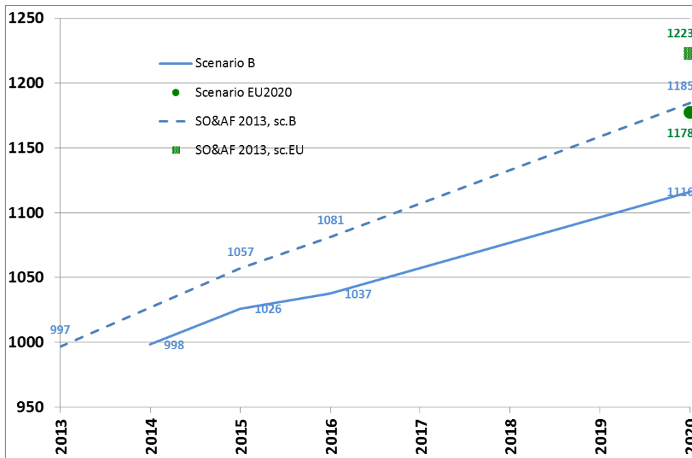
F. 3.2.1.2 – Comparison of NGC between SO&AF 2013 and SO&AF 2014; scenarios B and EU2020; January 7 p.m. [GW]
