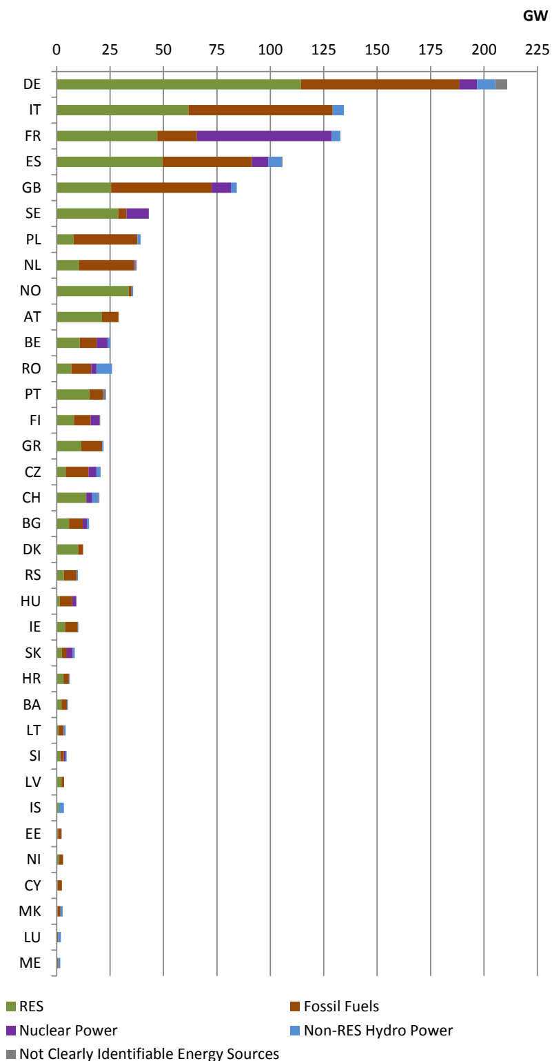
F. 3.2.1.6 – Total NGC breakdown per country in 2020; Scenario B; January 7 p.m.
