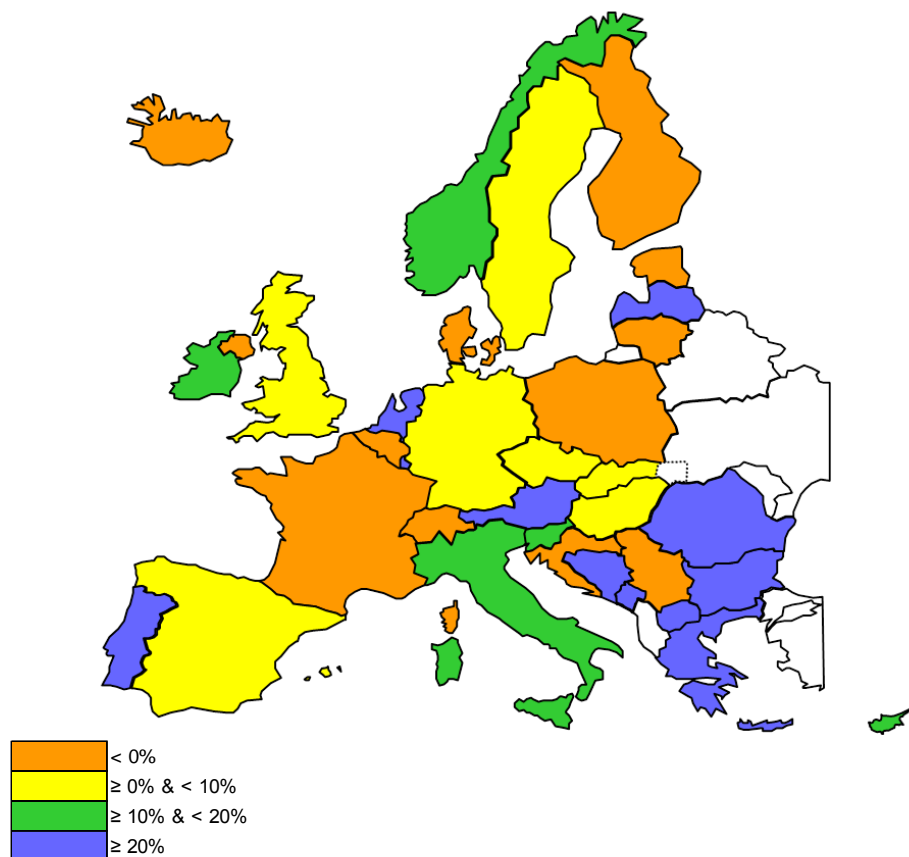
F 4.1.8 – Remaining Capacity minus Adequacy Reference Margin as a part of Reliably Available Capacity per country, Scenario B, January 2020, 7 p.m.
