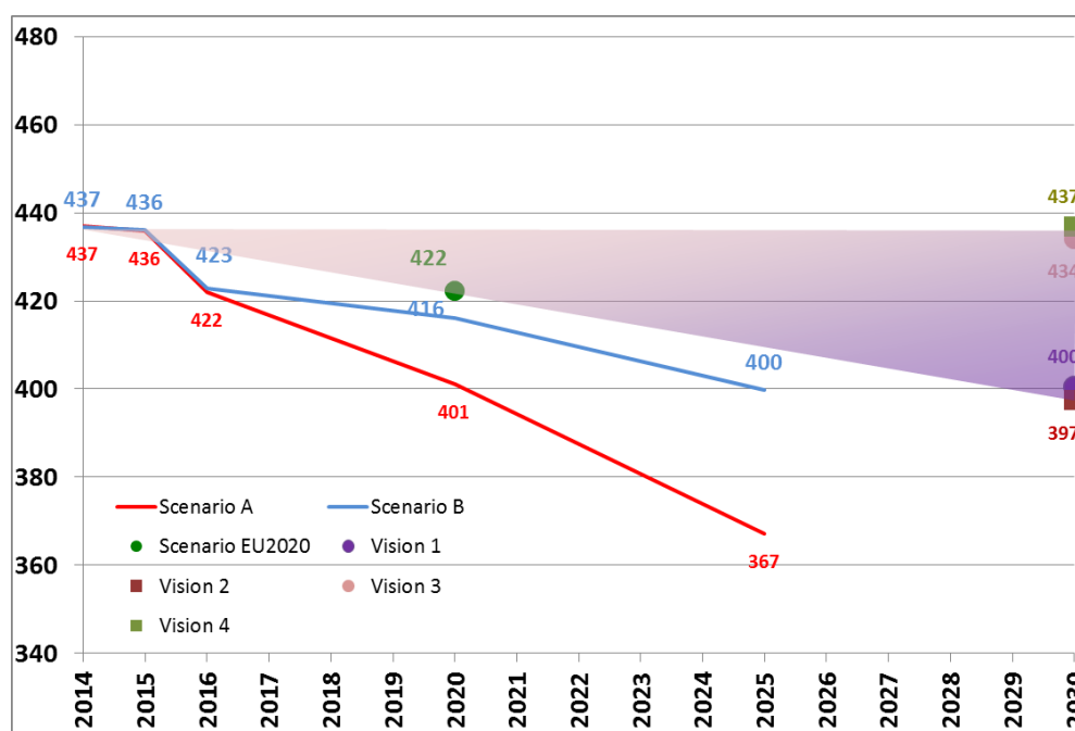
F. 3.2.2.1 - ENTSO-E Fossil fuels generation capacity forecast; all scenarios; January 7 p.m.. [GW]
