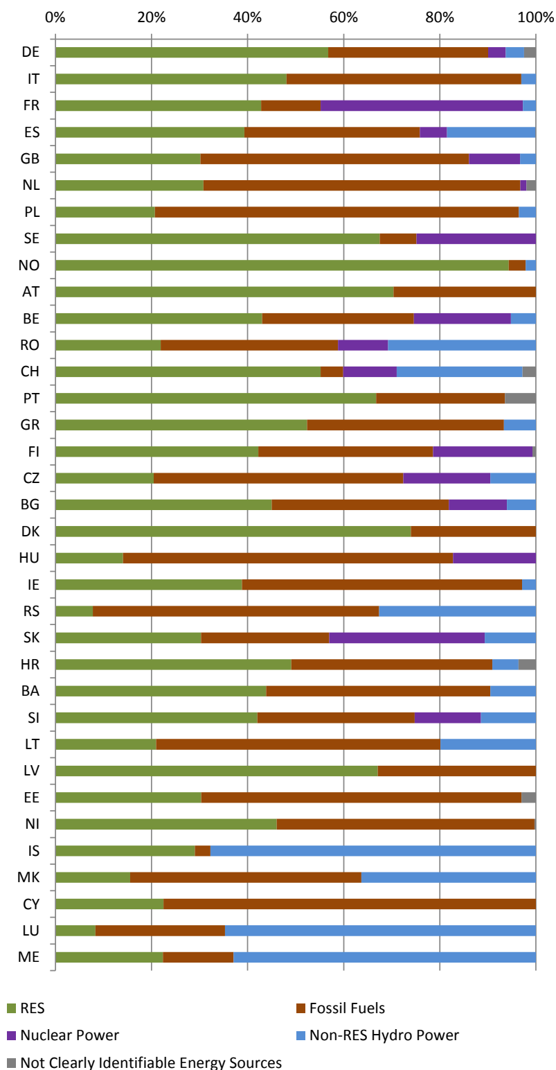
F. 3.2.1.11 – Total generation capacity mix per country in 2020; Scenario EU 2020; January 7 p.m.
