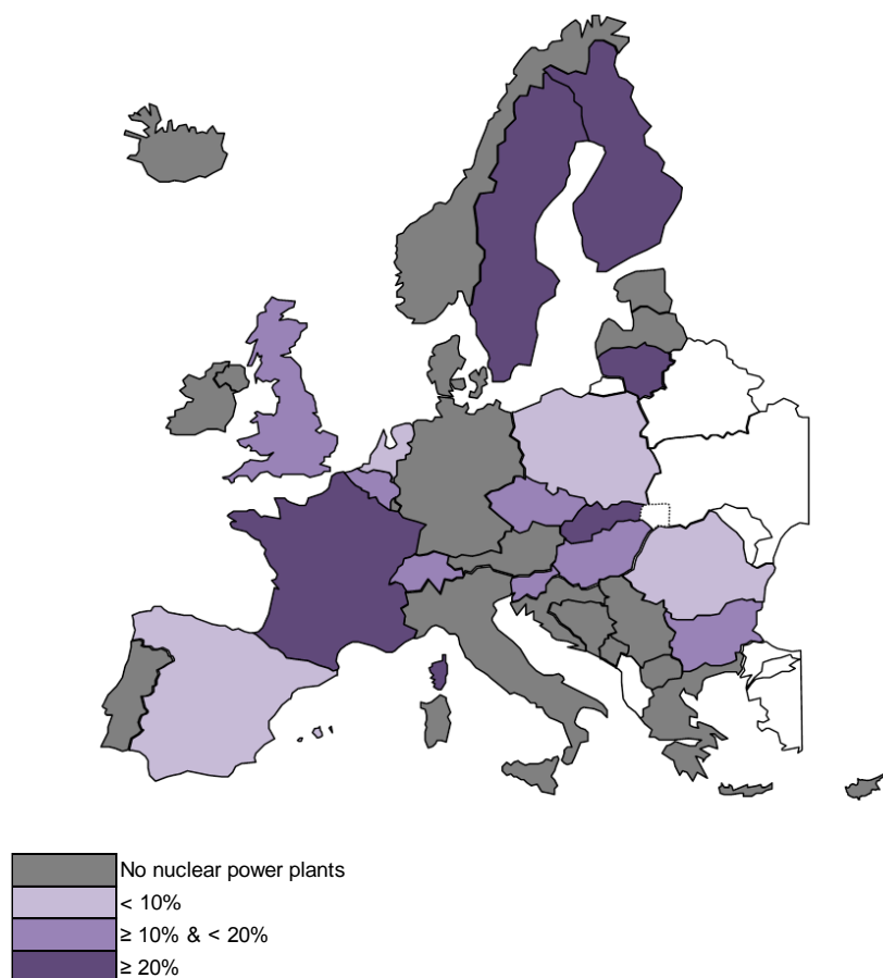
F 3.2.3.5 - Nuclear installed capacity as a part of NGC per country in 2025; Scenario B; January 7 p.m.
