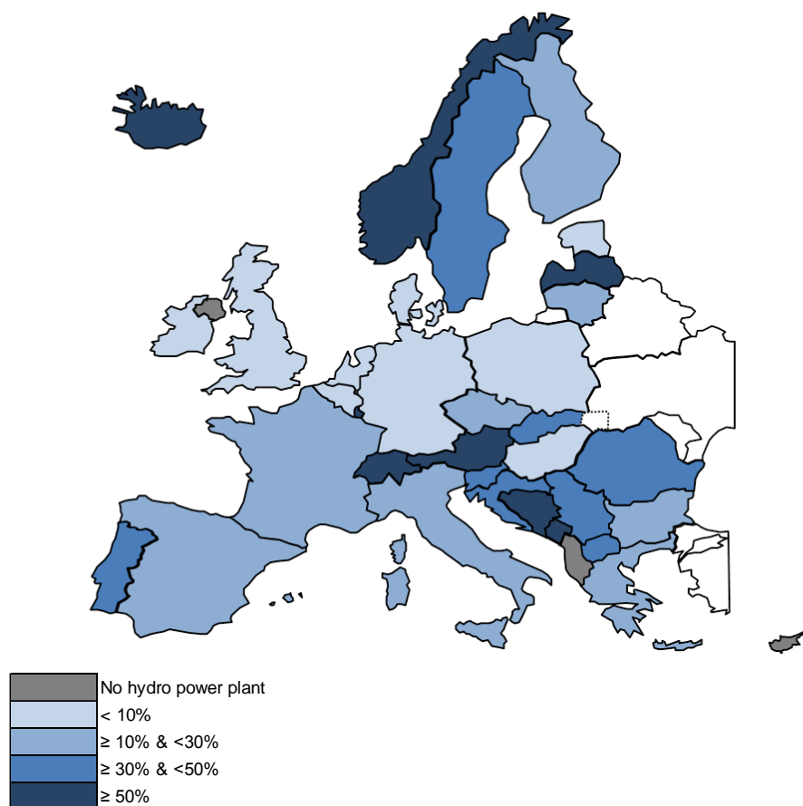
F. 3.2.5.5 – Total HPP installed capacity as part of NGC per country in 2014; Scenario B; January 7 p.m.
