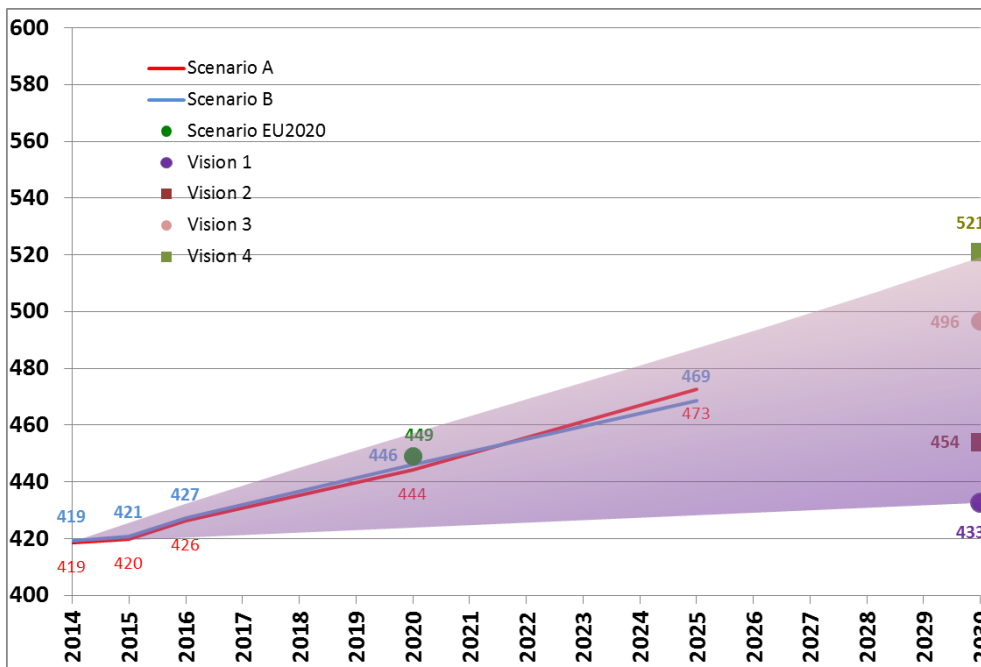
Figure 1.1b. Load (all Scenarios, July; GW)
