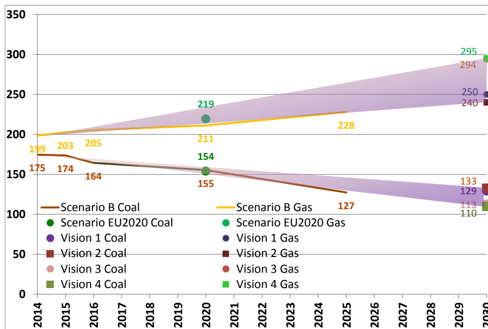
F. 3.2.2.3 – ENTSO-E Coal (hard coal+lignite) and Gas generation capacity forecast; all scenarios; January 7 p.m. [GW]
