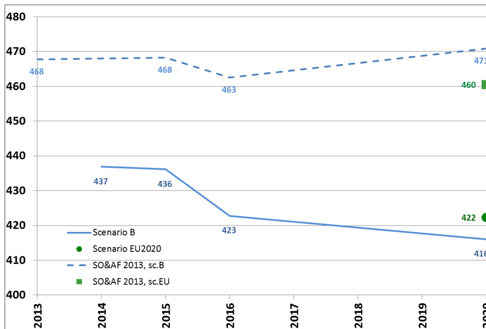
F. 3.2.2.2 – Comparison of Fossil fuels generation capacity between SO&AF 2013 and SO&AF 2014; scenarios B and EU2020; January 7 p.m. [GW]
