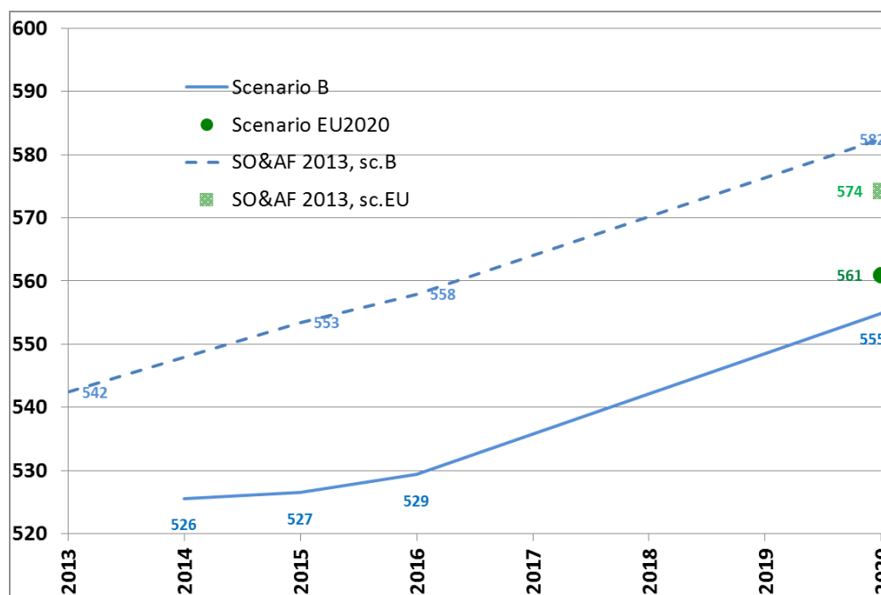
F. 3.1.3 – Differences between ENTSO-E load forecast in SO&AF 2013-2030 and in SO&AF 2014-2030 for scenario B and EU2020 in January [GW]
