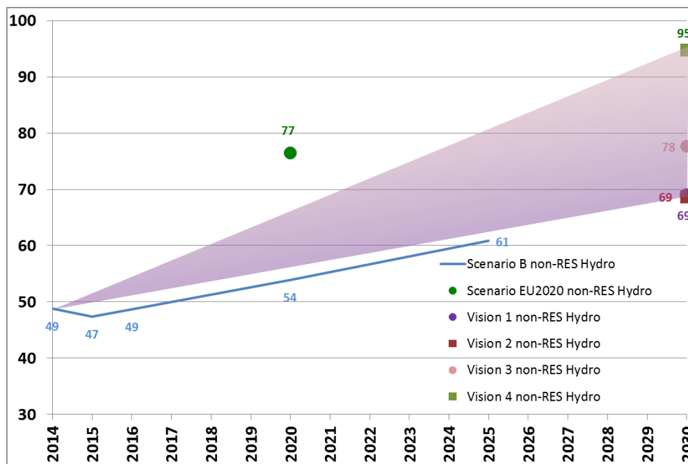
F. 3.2.5.3 – ENTSO-E non-RES HPP generation capacity forecast; all scenarios; January 7 p.m. [GW]
