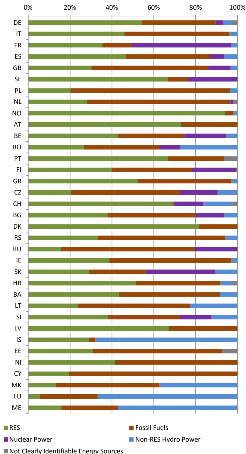
F. 3.2.1.8 – Total generation capacity mix per country in 2020; Scenario B; January 7 p.m.
