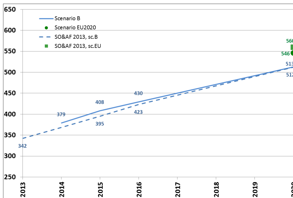
F. 3.2.4.2 – Comparison of RES generation capacity between SO&AF 2013 and SO&AF 2014; Scenarios B and EU2020; January 7 p.m. [GW]
