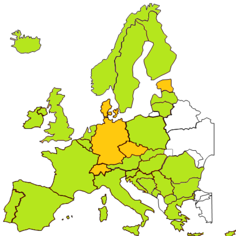
Figure 4.2.1: Remaining Capacity minus Adequacy Reference Margin; Scenario B; January 2025
