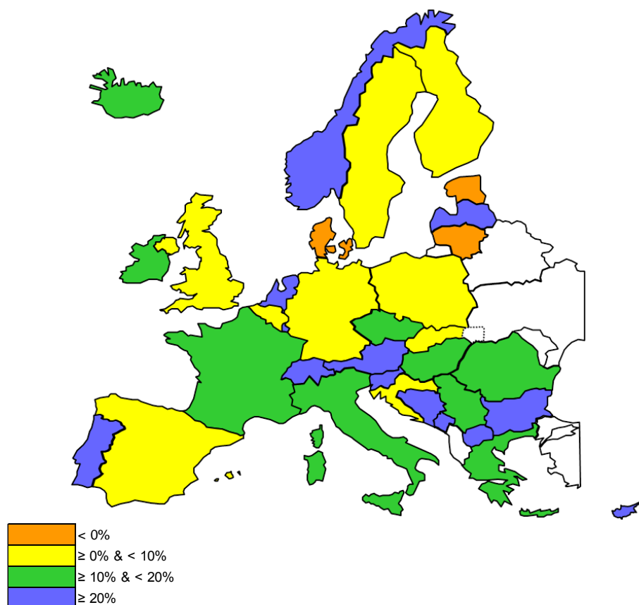
F 4.1.10 – RC as a part of NGC per country – Scenario EU 2020, reference point January
