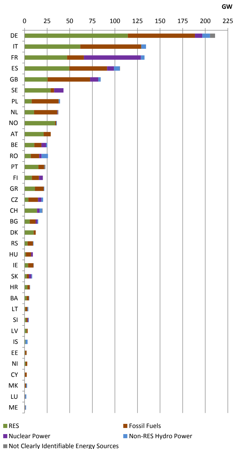
F. 3.2.1.7 – Total NGC breakdown per country in 2025; Scenario B; January 7 p.m.
