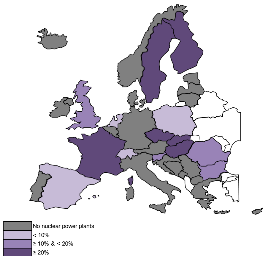
F 3.2.3.6 - Nuclear installed capacity as a part of NGC per country in 2030; Vision 1; January 7 p.m.
