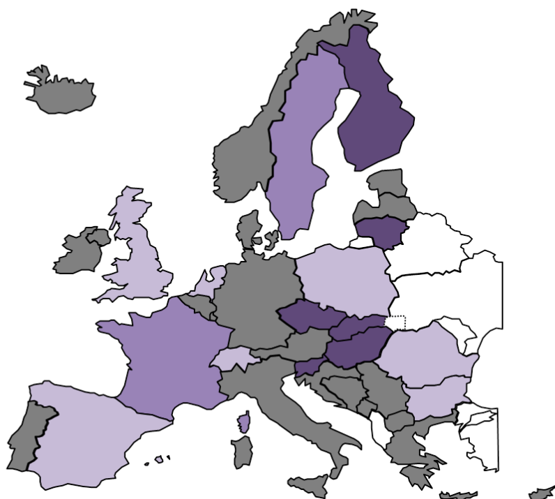
F 3.2.3.7 - Nuclear installed capacity as a part of NGC per country in 2030; Vision 4; January 7 p.m.
