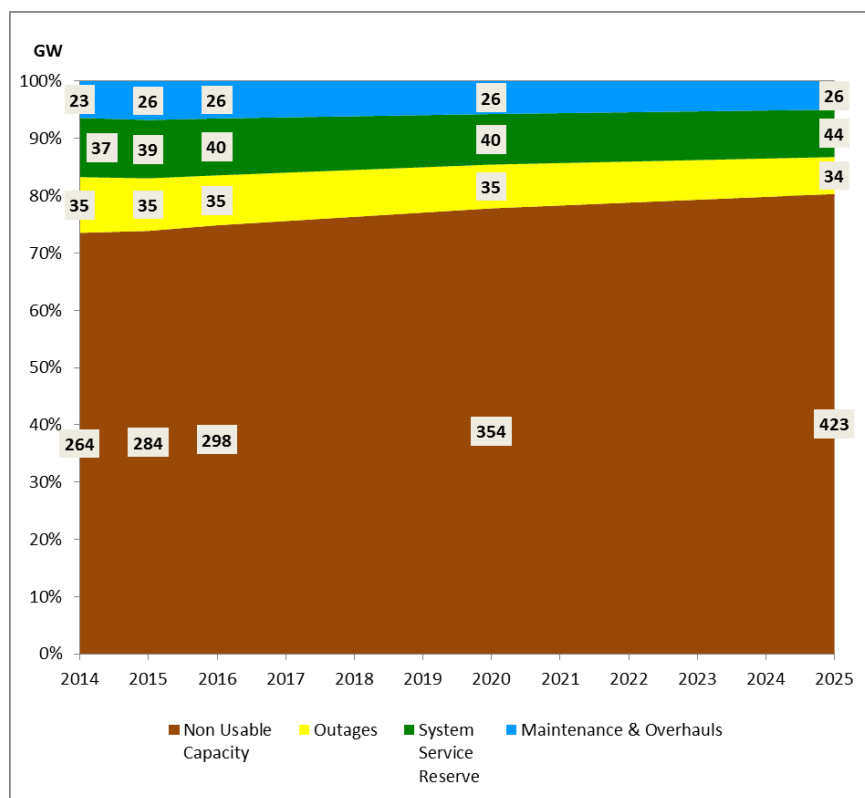
F. 3.3.5 – ENTSO-E UC mix, scenario B, January
