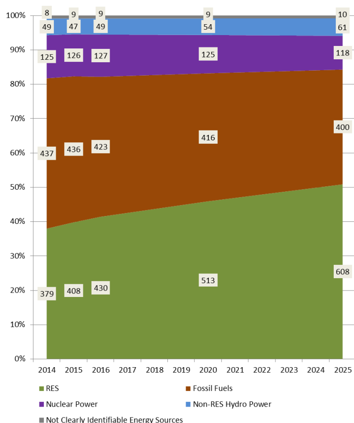
Figure 1.3: ENTSO-E total NGC breakdown per fuel type (all years; Scenario B; January 7 p.m.)
