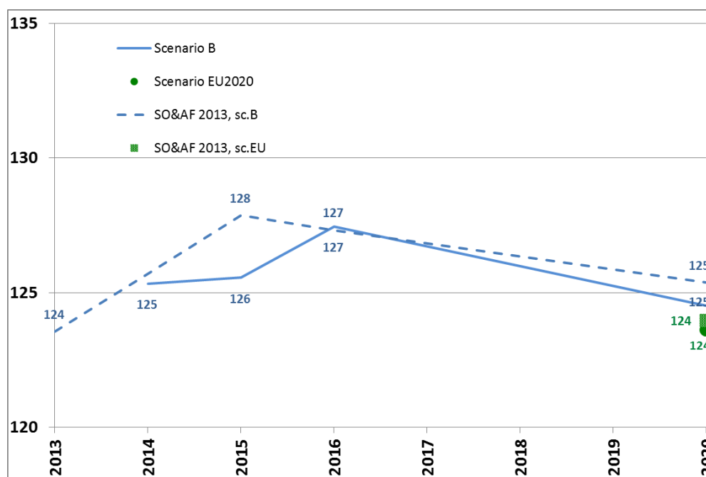
F. 3.2.3.2 – Comparison of nuclear generation capacity between SO&AF 2013 and SO&AF 2014; Scenarios B and EU2020; January 7 p.m. [GW]
