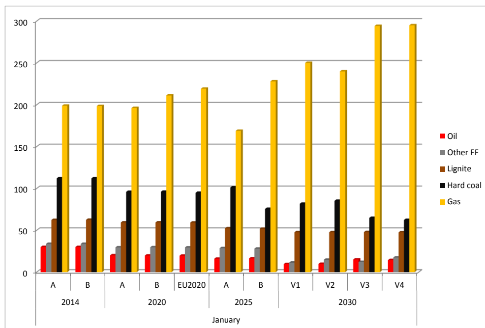
F. 3.2.2.4 - ENTSO-E Fossil fuels generation capacity breakdown in 2014, 2020 and 2030; all scenarios; January 7 p.m. (ratios and absolute values in GW)
