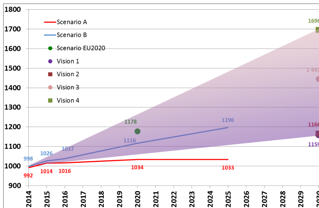
F. 3.2.1.1 - ENTSO-E total NGC forecast; all scenarios; January 7 p.m. [GW]
