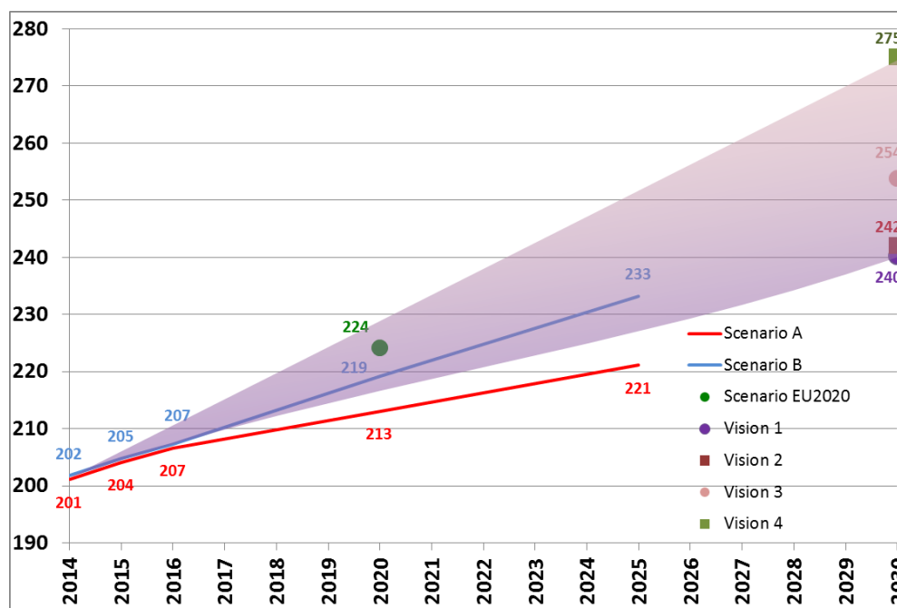
F. 3.2.5.1 – ENTSO-E total HPP generation capacity forecast; all scenarios; January 7 p.m. [GW]
