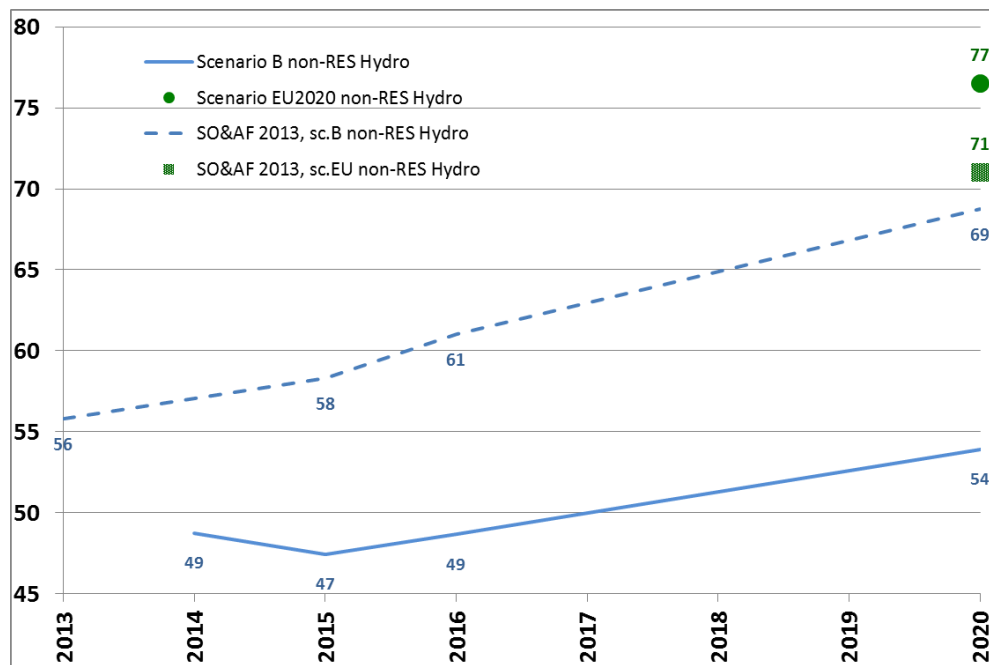
F 3.2.5.4 – Comparison of non-RES HPP generation capacity between SO&AF 2013 and SO&AF 2014; Scenarios B and EU2020; January 7 p.m. [GW]
