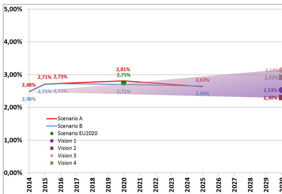
F. 3.1.11 - ENTSO-E load management trends for all scenarios in January [%]
