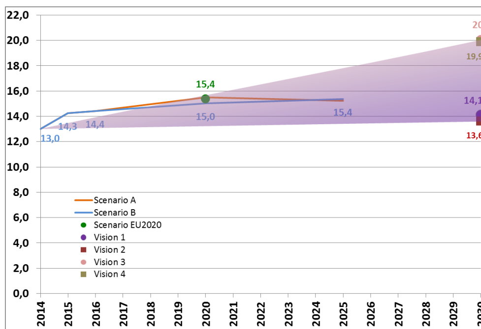
F. 3.1.10 - ENTSO-E load management trends for all scenarios in January [GW]
