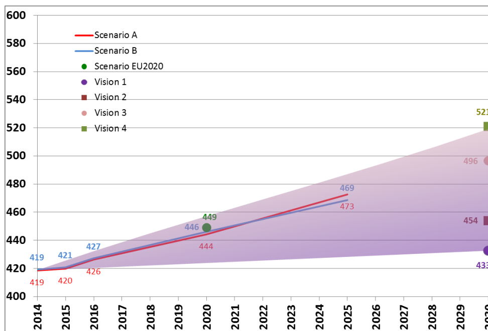
F. 3.1.2. - ENTSO-E load forecast for all scenarios in July [GW]
