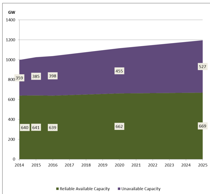
F. 3.3.6 – ENTSO-E UC and RAC forecast, scenario B, January 7 p.m. [GW]
