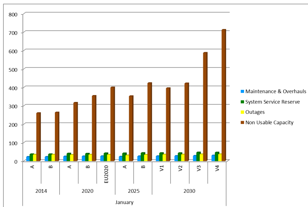
F. 3.3.4 – ENTSO-E UC forecast, January [GW]
