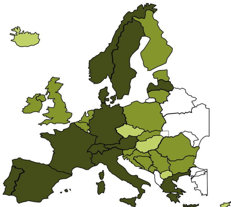
F. 3.2.4.10 – RES installed capacity as part of NGC per country in 2030; Vision 4; January 7 p.m.
