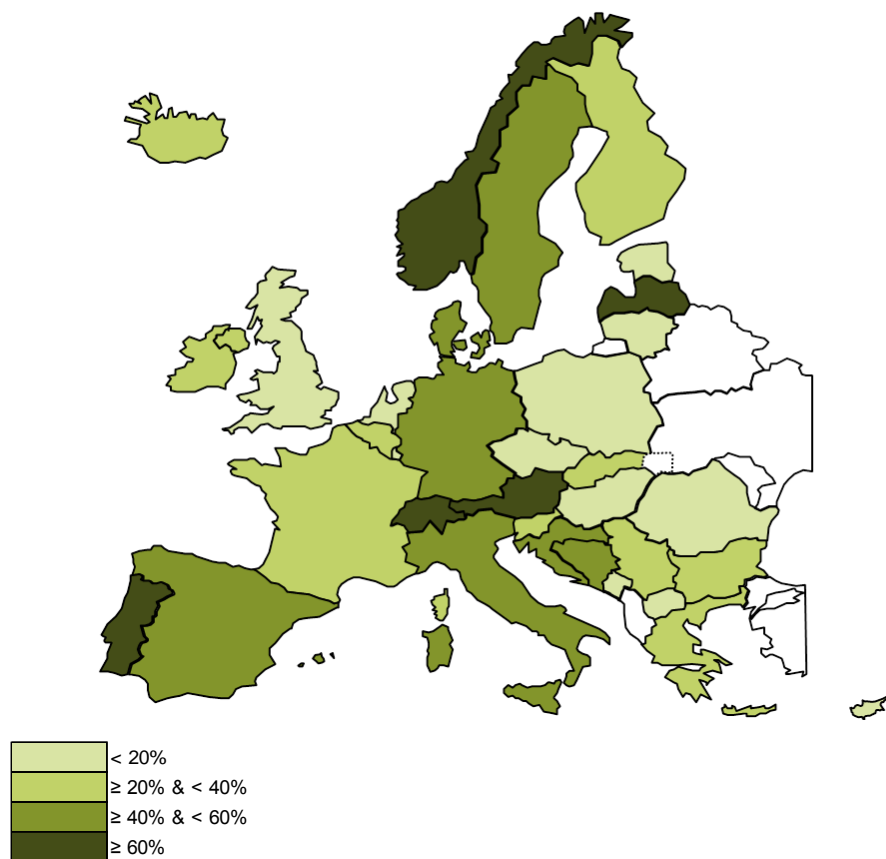
F. 3.2.4.5 – RES installed capacity as part of NGC per country in 2014; Scenario B; January 7 p.m.
