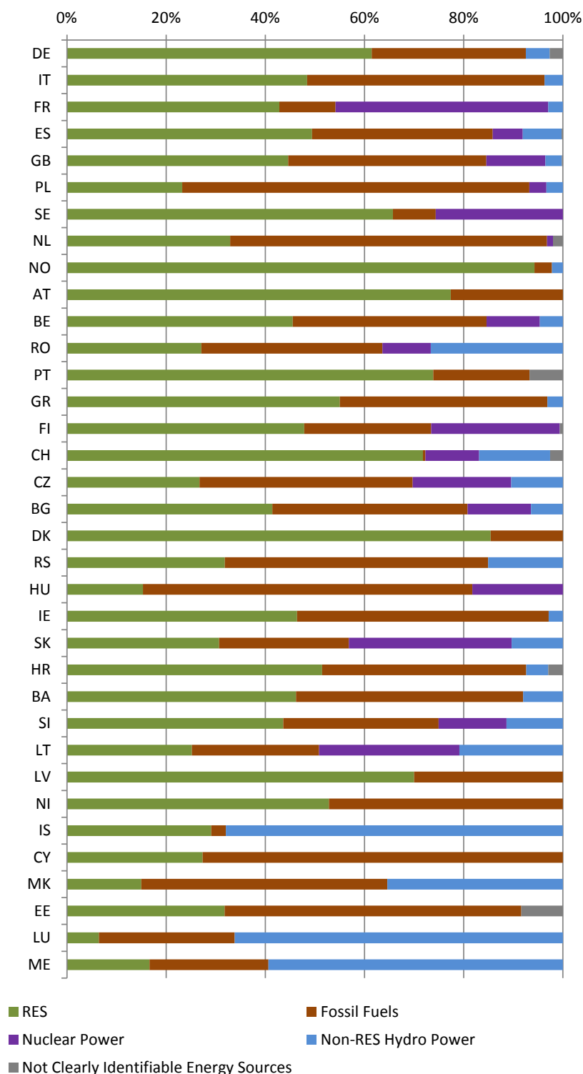
F. 3.2.1.9 – Total generation capacity mix per country in 2025; Scenario B; January 7 p.m.
