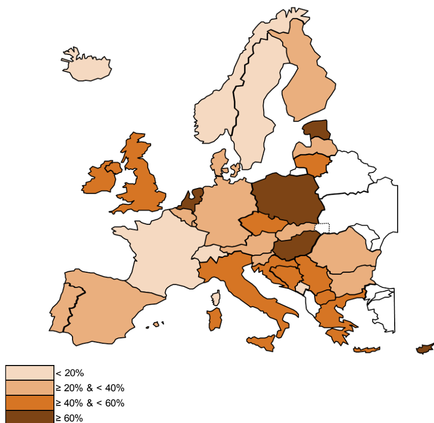
F. 3.2.2.8 - Fossil fuels installed capacity as a part of NGC per country in 2020; Scenario EU 2020; January 7 p.m.
