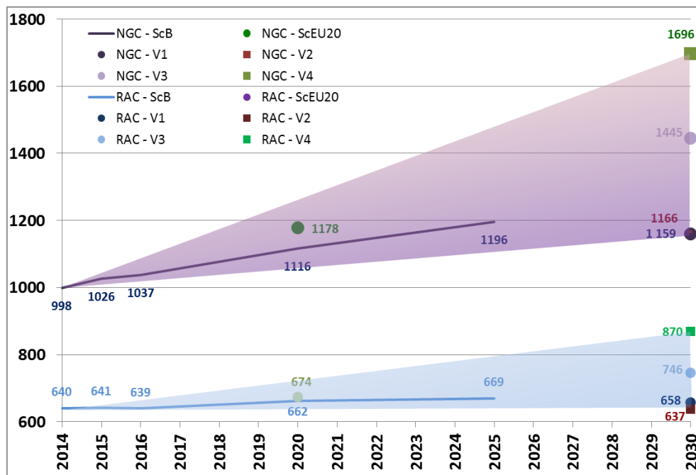
F. 3.3.3 – ENTSO-E NGC & RAC forecast in scenarios B, EU2020 and Visions, January [GW]
