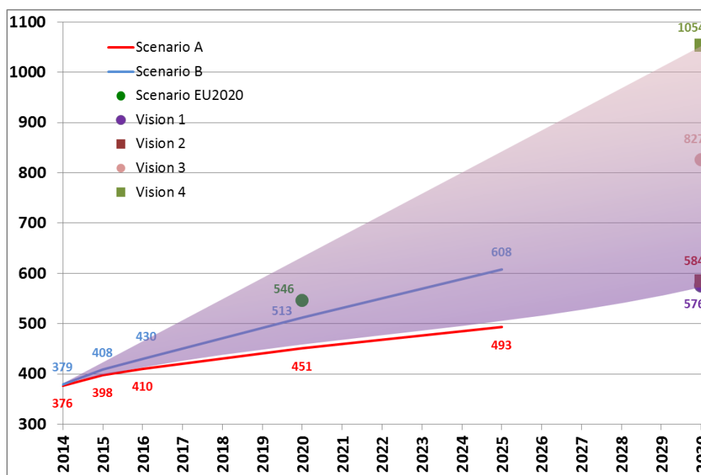
F. 3.2.4.1 – ENTSO-E RES generation capacity forecast; all scenarios; January 7 p.m. [GW]
