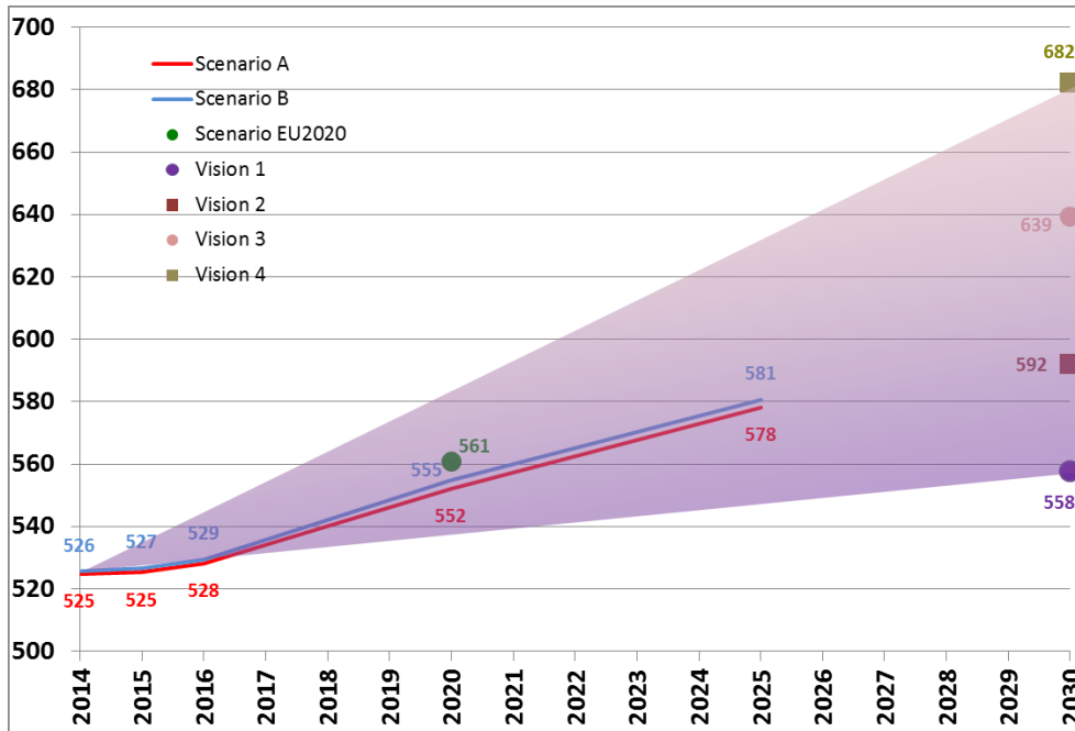
Figure 1.1a. Load (all Scenarios, January; GW)
