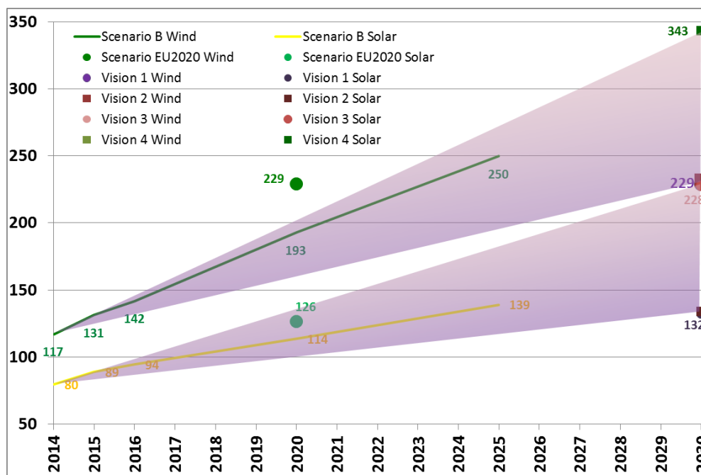
F. 3.2.4.4 – ENTSO-E Wind and Solar generation capacity forecast; all scenarios; January 7 p.m. [GW]
