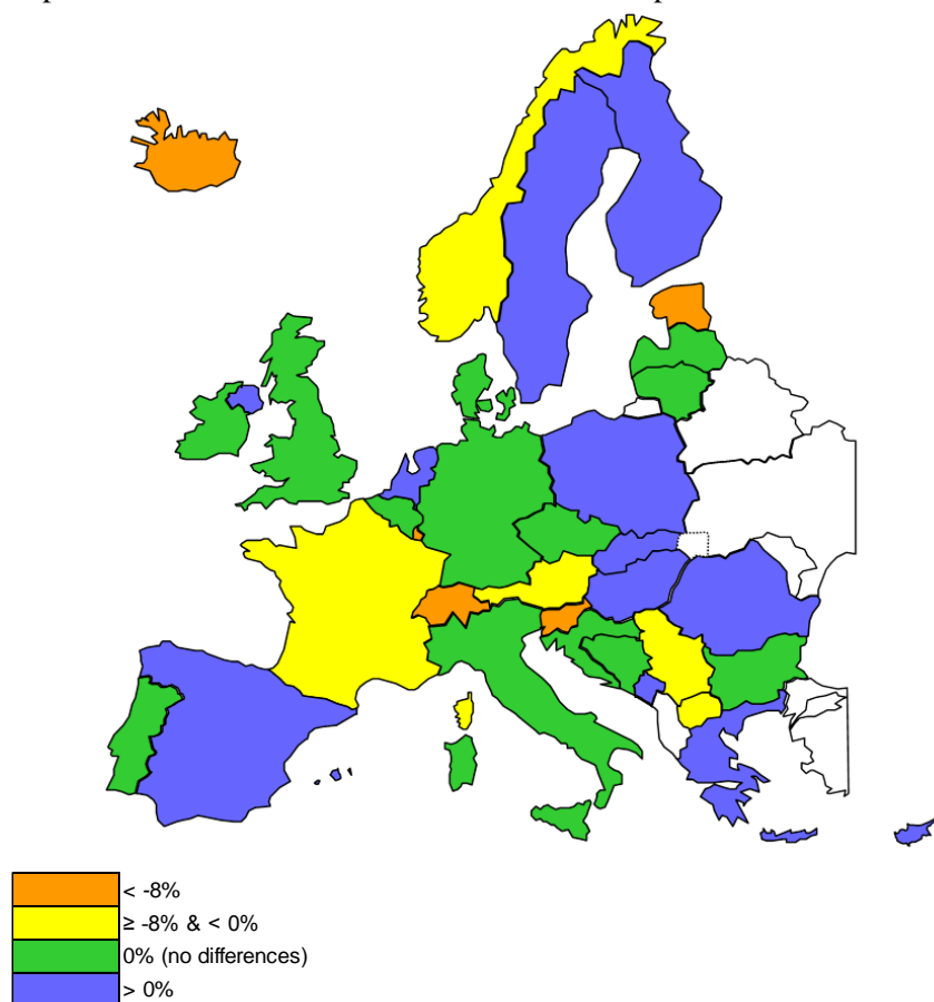
F 3.1.5 - Difference of ENTSO-E load in 2020 in Scenario EU 2020 with relation to Scenario B, January
